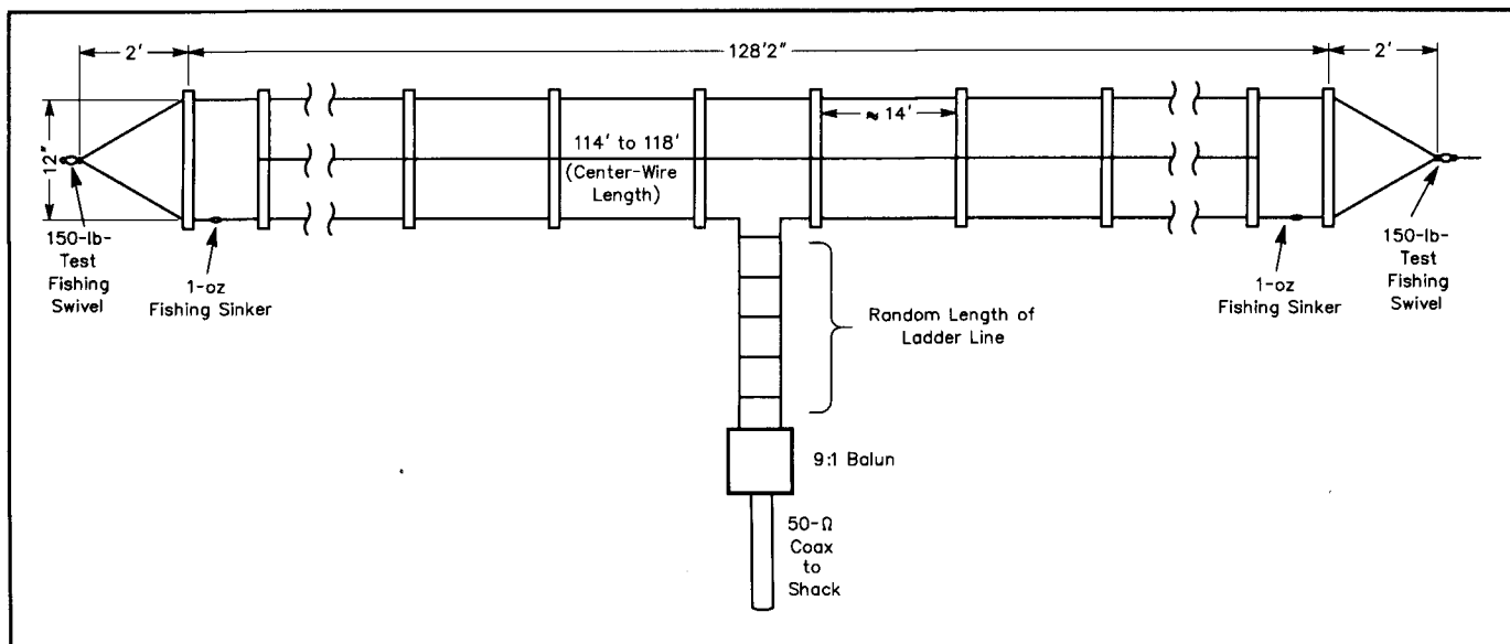
Figure 3—The open-sleeve folded dipole: simple and inexpensive. The antenna is fed with a random length of 450- \Omega open-wire transmission line through a 9:1 balun.
